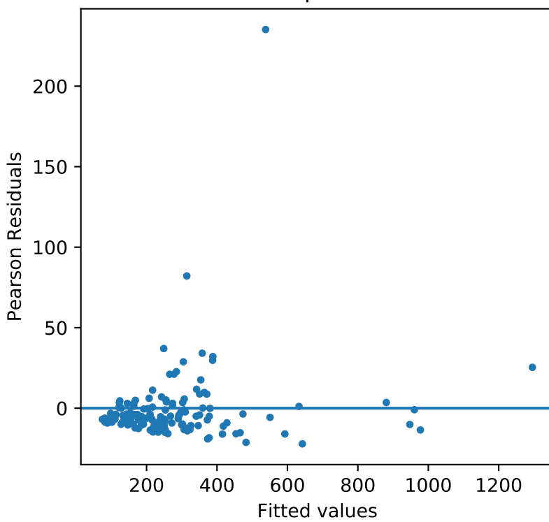
Residual Dependence Plot
