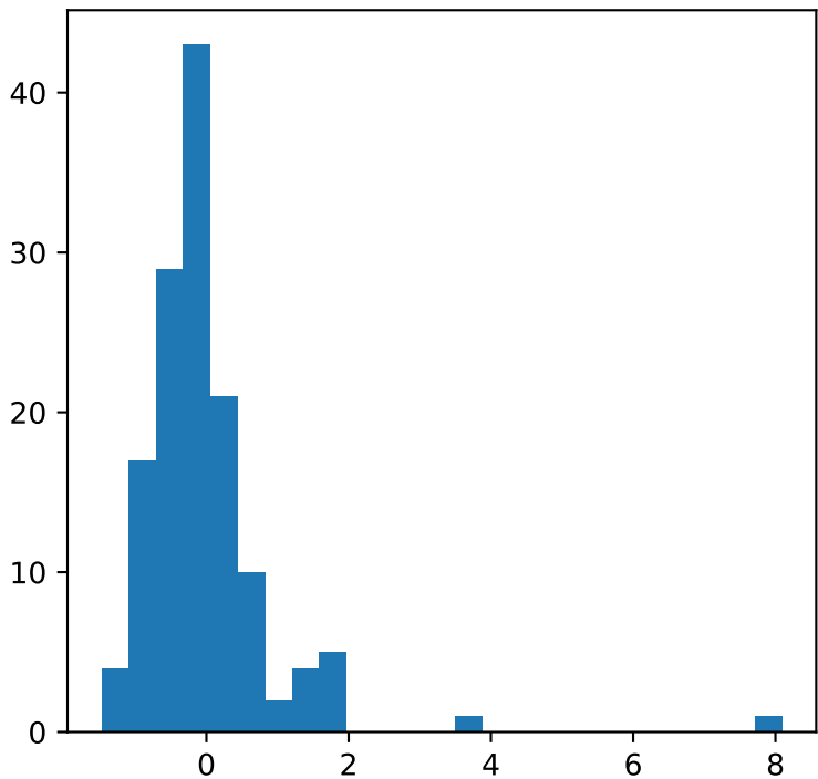
Histogram of standardized deviance residuals
