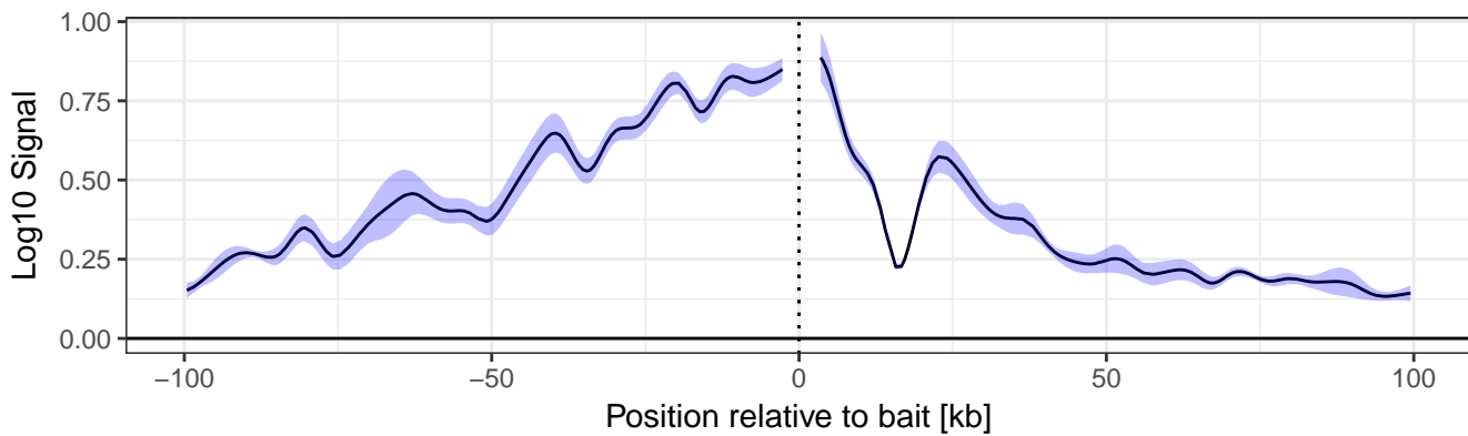
Mean log10 4C signal
